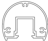
Excell Round Top Rail (Component Glass) HEIGHT: 1 15/16" WIDTH: 2 1/4" ALLOY: 6063-T5
