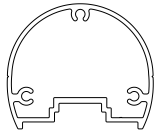
Excell Round Top Rail (Component Glass) HEIGHT: 2 5/32" WIDTH: 3 21/32" ALLOY: 6063-T5
