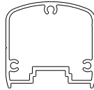
Excell Square Top Rail (Welded Picket) HEIGHT: 2 5/32" WIDTH: 3 21/32" ALLOY: 6063-T5
