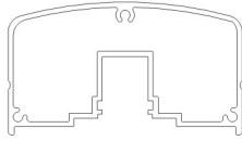
Excell Park Rail Top Rail (Component Glass) HEIGHT: 2" WIDTH: 3 1/2" ALLOY: 6063-T5
