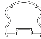
Excell Heritage Top Rail (Welded Picket) HEIGHT: 1 15/16" WIDTH: 2" ALLOY: 6063-T5
