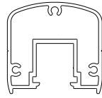
Excell Square Top Rail (Component Glass) HEIGHT: 1 15/16" WIDTH: 2" ALLOY: 6063-T5
