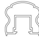
Excell Heritage Top Rail (Component Glass) HEIGHT: 1 15/16" WIDTH: 2" ALLOY: 6063-T5
