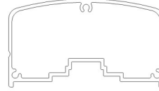
Excell Park Rail Top Rail (Welded Picket) HEIGHT: 2" WIDTH: 3 1/2" ALLOY: 6063-T5
