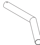
1.9" or 1.6" Pipe Mitered 143° 12"x12" (for 37° Stairs)
