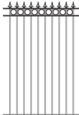
Fence Style 08
